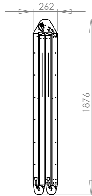
FRAME IN FOLDED DOWN VIEW
